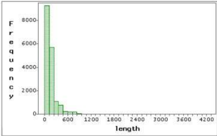
Figure 2. Peptide precursor protein length distribution
