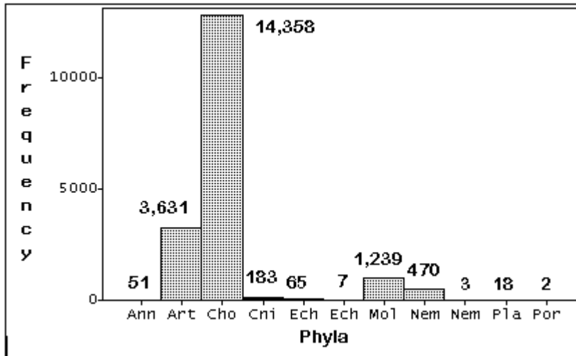
Fig. 3. Peptide frequency distribution among phyla.
