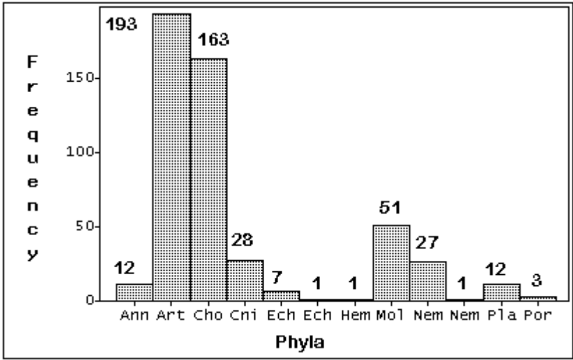
Fig. 4. Peptide family frequency distribution among phyla.
